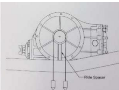
FIG. 31 Squaring marks on MK2 chassis.
