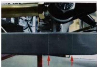
FIG. 31 Squaring marks on MK2 chassis.
